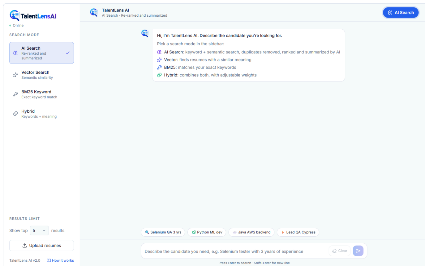
Figure 1. Home screen
