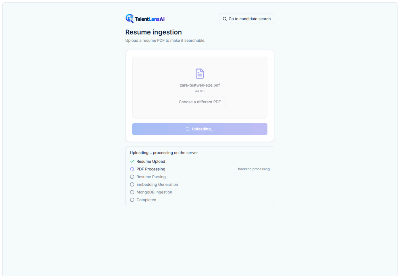
Figure 17. Ingestion in progress
