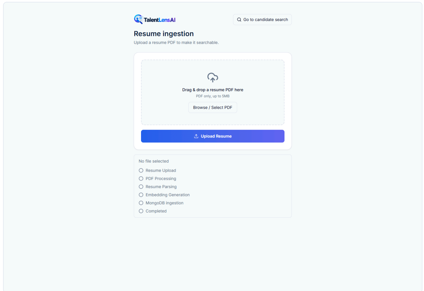
Figure 15. Upload page
