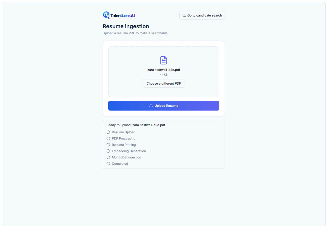
Figure 16. File selected
