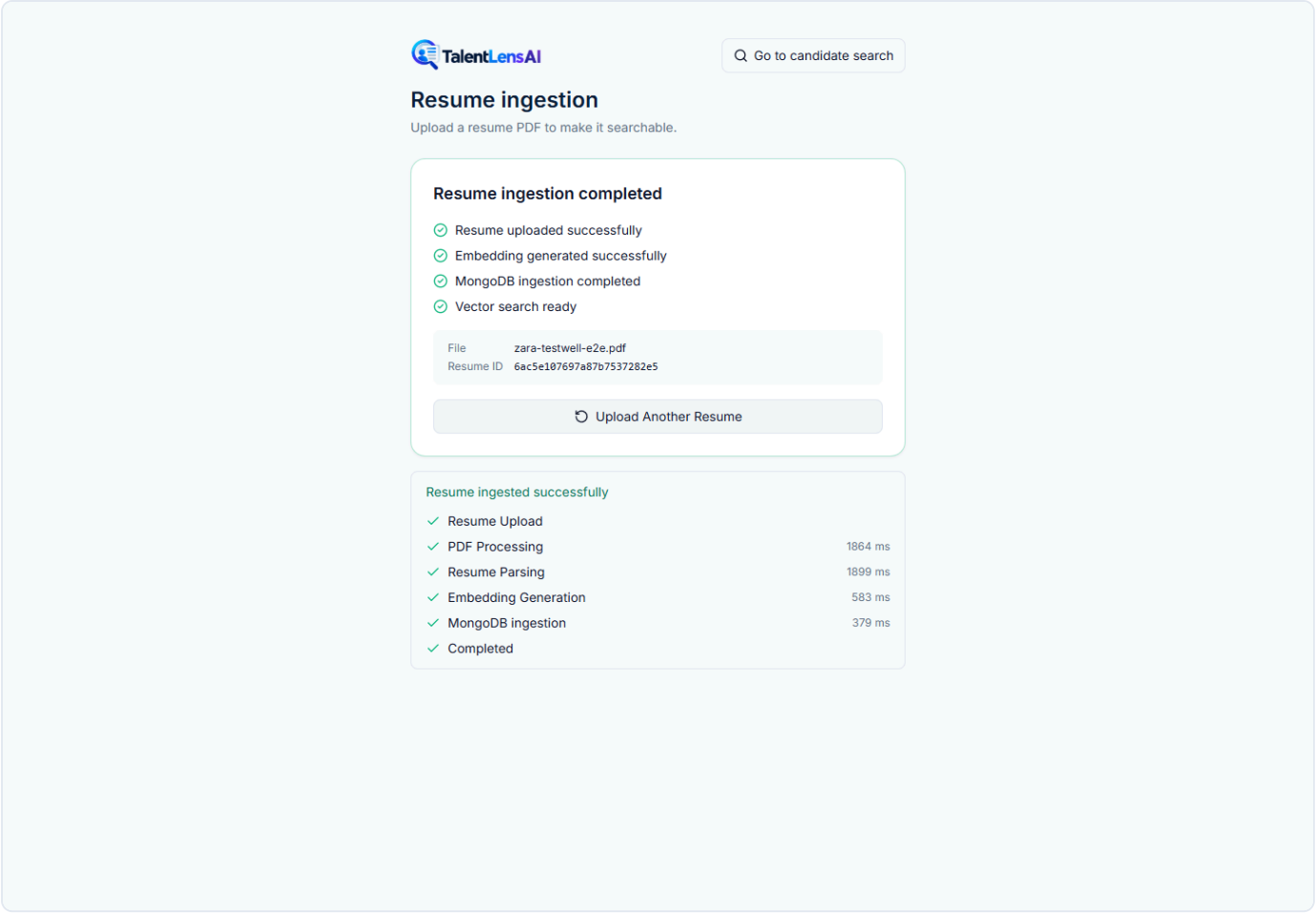
Figure 18. Ingestion completed
